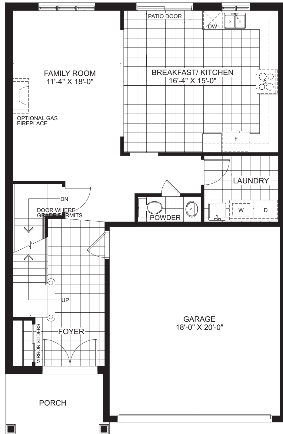
Ground Floor – Elevation A & B
