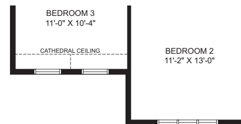
Second Floor – Elevation B
